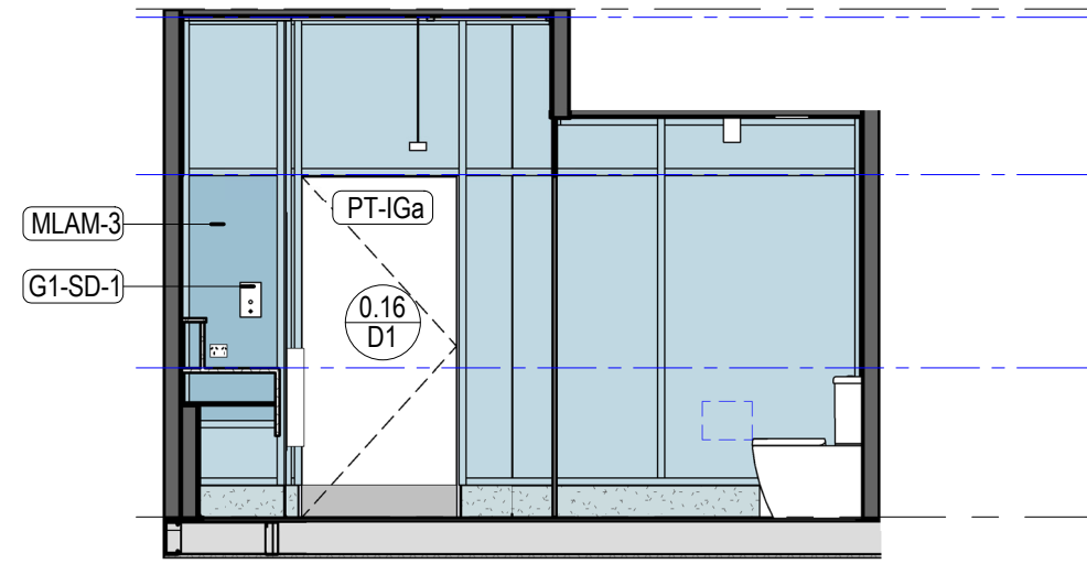
3 0.15 - Female - North Elevation 1 : 50
