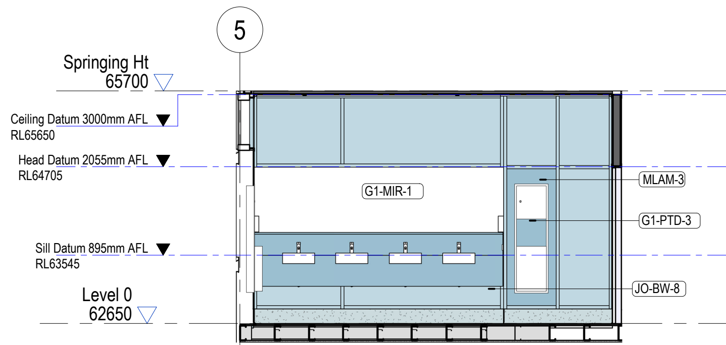
2 0.15 - Female - West Elevation 1 : 50
