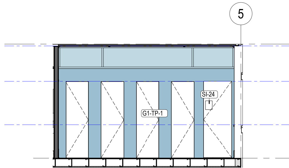
5 0.15 - Female - East Elevation 1 1 : 50
