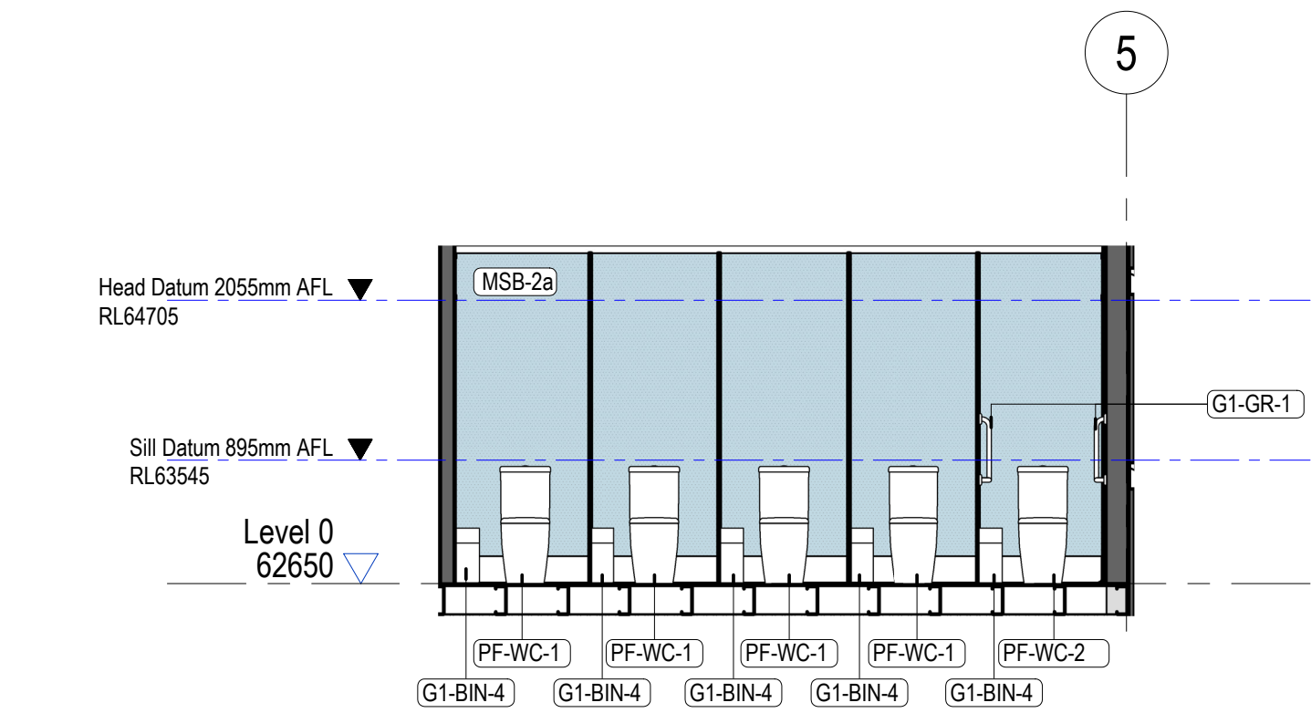
6 0.15 - Female - East Elevation 2 1 : 50
